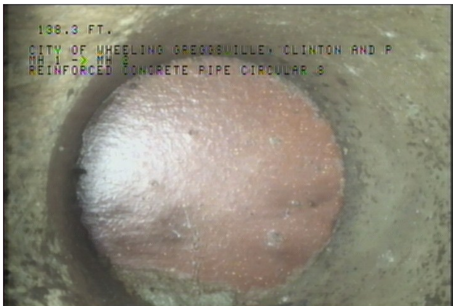
4, 00:04:56, 138.30ft Tap Factory Made Capped, at 09 o'clock, -, within 8 inches of joint: YES, 6"
