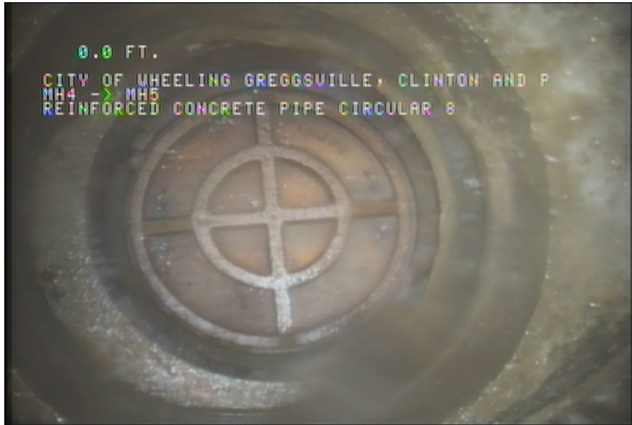
1, 00:00:00, 0.00ft Upstream Manhole, Survey Begins / MH4
