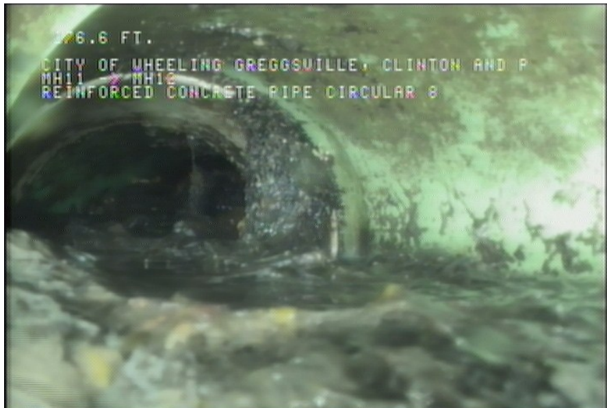
8, 00:21:20, 276.60ft Tap Factory Made, at 09 o'clock, -, within 8 inches of joint: YES, 4" / HOUSE NUMBER 202
