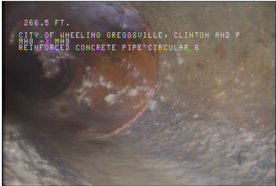
5, 00:13:13, 266.50ft Tap Factory Made, at 09 o'clock, -, within 8 inches of joint: YES, 6" / HOUSE NUMBER 230
