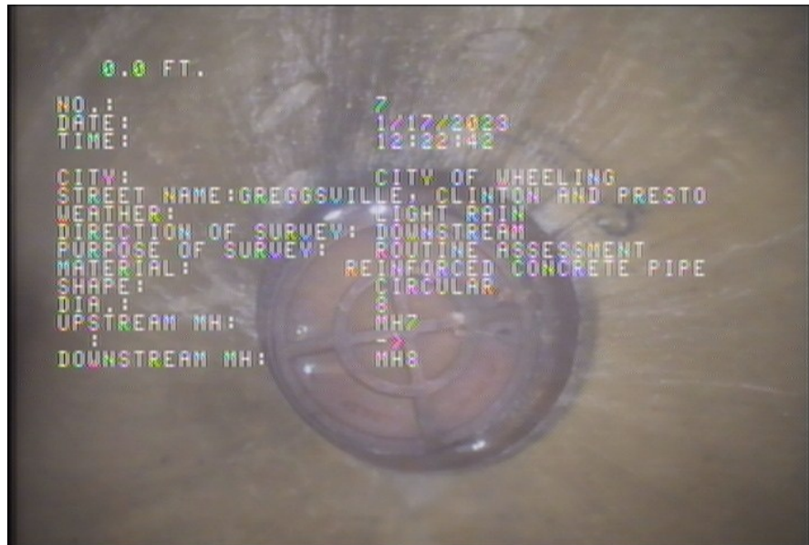
1, 00:00:00, 0.00ft Upstream Manhole, Survey Begins / MH7
