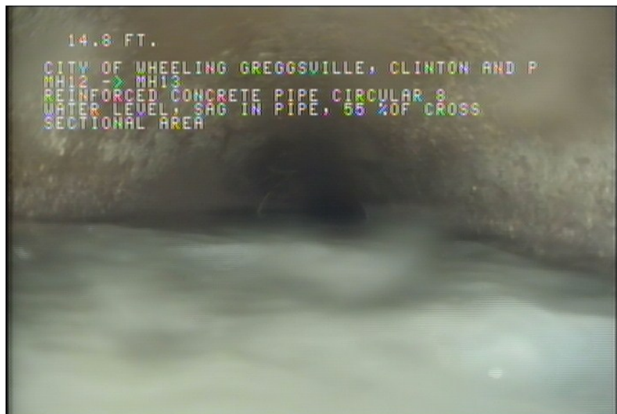
2, 00:04:53, 14.80ft Water Level, Sag in pipe, 55 %of cross sectional area
