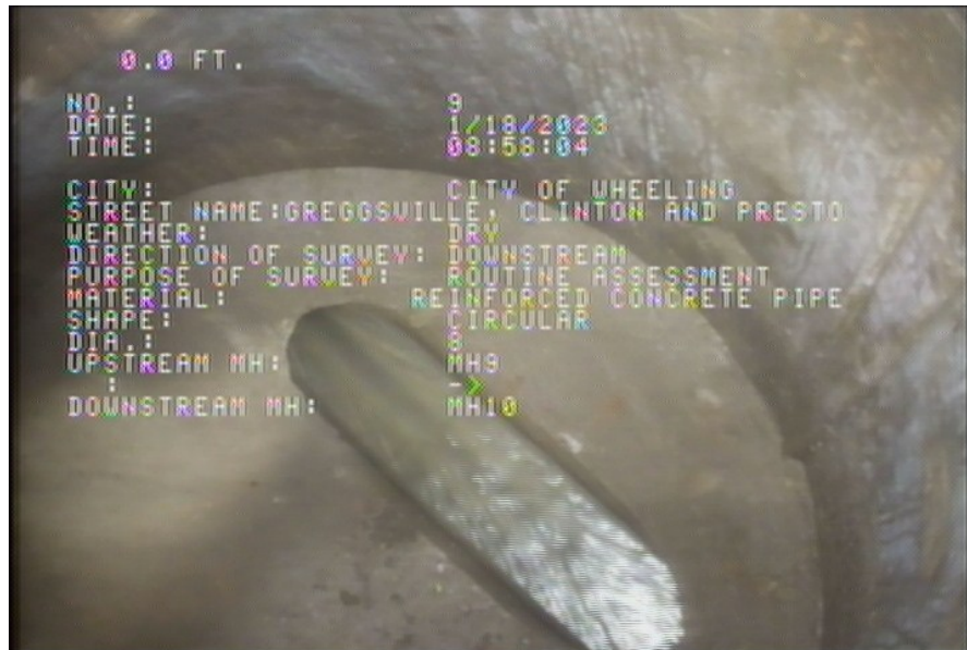
1, 00:00:00, 0.00ft Upstream Manhole, Survey Begins / MH9
