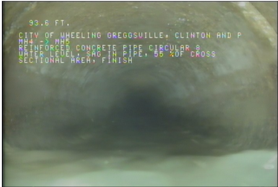
3, 00:05:52, 93.60ft Water Level, Sag in pipe, 55 %of cross sectional area, Finish
