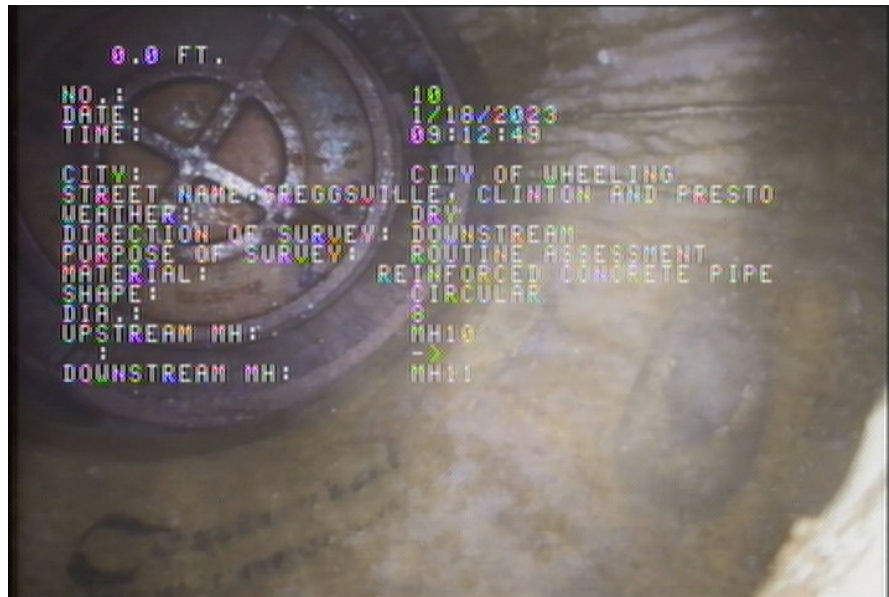
1, 00:00:00, 0.00ft Upstream Manhole, Survey Begins / MH10
