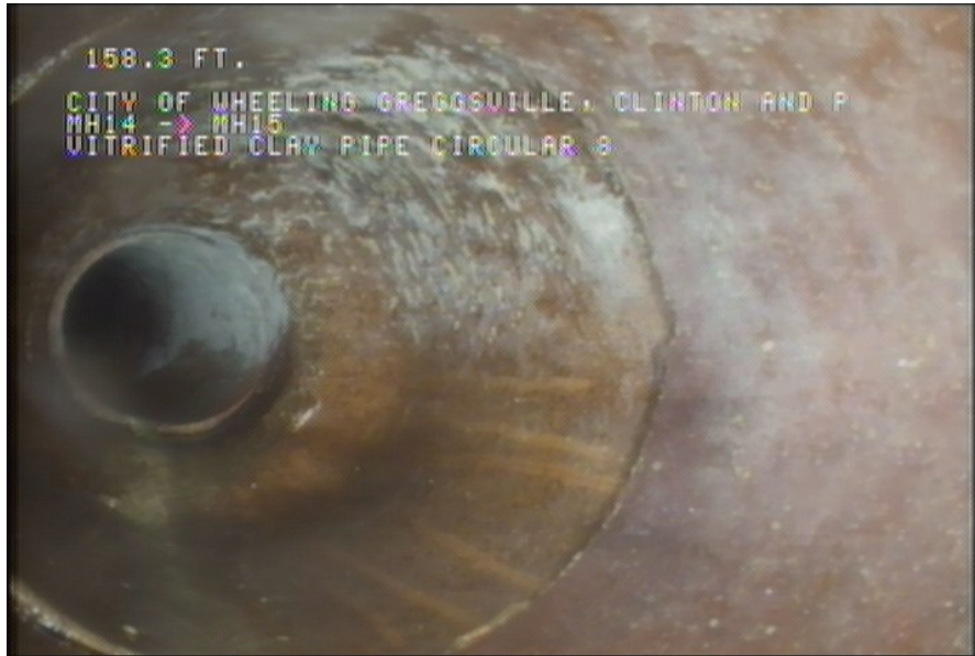
5, 00:15:04, 158.30ft Tap Factory Made, at 09 o'clock, -, within 8 inches of joint: YES, 6" / HOUSE NUMBER 152
