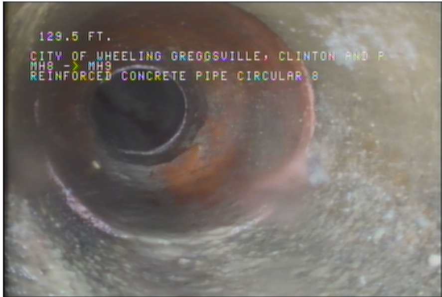
3, 00:06:11, 129.50ft Tap Factory Made, at 09 o'clock, -, within 8 inches of joint: YES, 6" / HOUSE NUMBER 234
