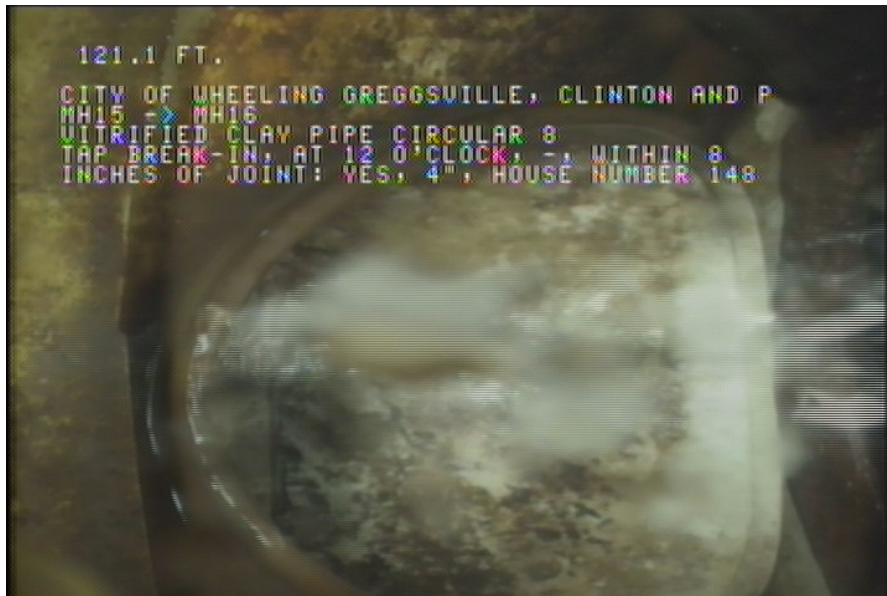
4, 00:09:11, 121.10ft Tap Break-In, at 12 o'clock, -, within 8 inches of joint: YES, 4" / HOUSE NUMBER 148
