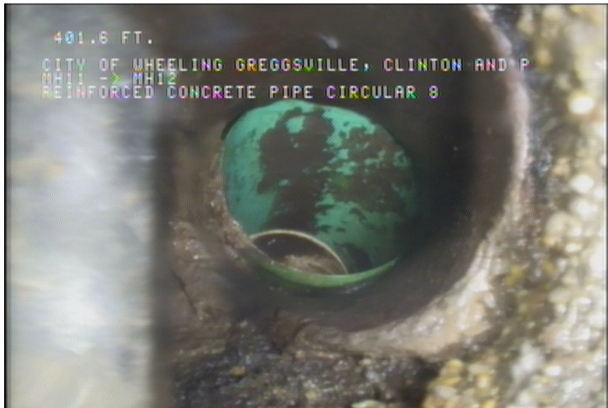
10, 00:31:10, 401.10ft Tap Break-In, at 12 o'clock, -, within 8 inches of joint: YES, 4" / HOUSE NUMBER 200
