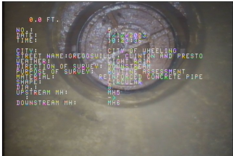
1, 00:00:00, 0.00ft Upstream Manhole, Survey Begins / MH5
