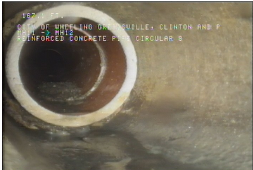
6, 00:13:23, 167.10ft Tap Factory Made, at 09 o'clock, -, within 8 inches of joint: YES, 6"
