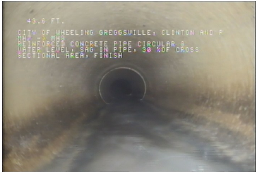
3, 00:03:17, 43.60ft Water Level, Sag in pipe, 30 % of cross sectional area, Finish
