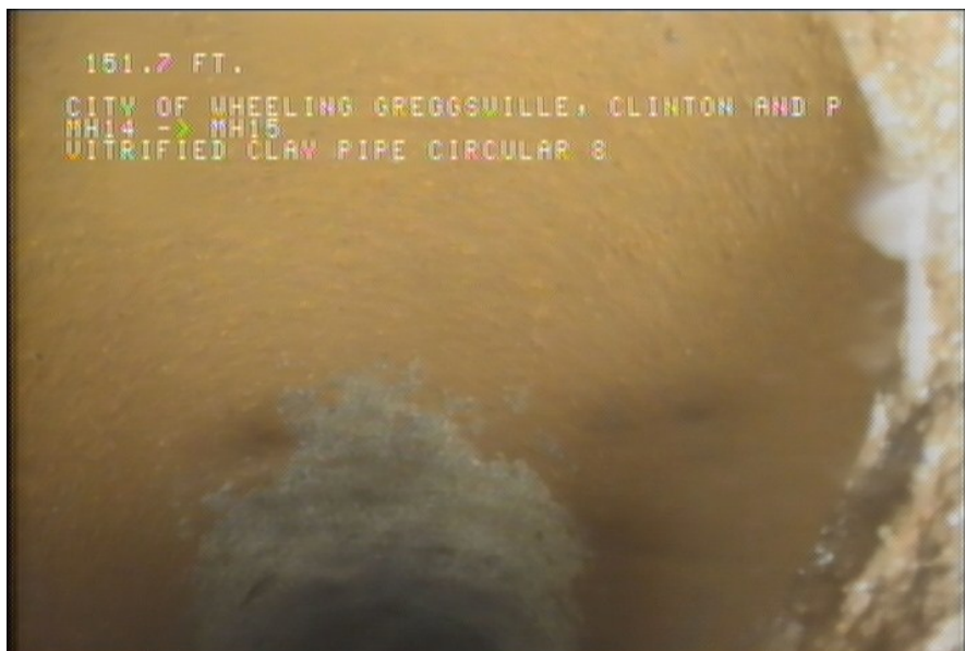
4, 00:12:49, 151.70ft Tap Break-In, at 10 o'clock, -, within 8 inches of joint: YES, 4" / HOUSE NUMBER 154
