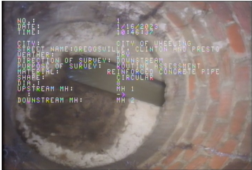
1, 00:00:00, 0.00ft Upstream Manhole, Survey Begins / MH 1
