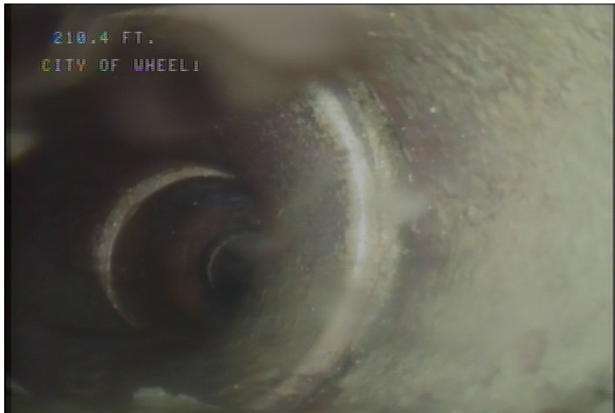
6, 00:17:15, 210.40ft Tap Factory Made, at 09 o'clock, -, within 8 inches of joint: YES, 6" / HOUSE NUMBER 152
