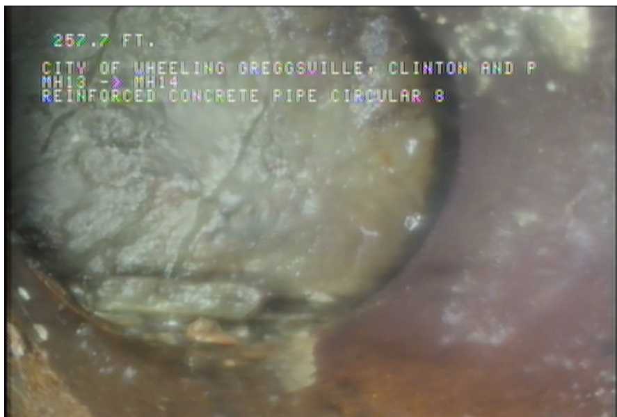
6, 00:19:56, 257.70ft Tap Factory Made Capped, at 09 o'clock, -, within 8 inches of joint: YES, 6"
