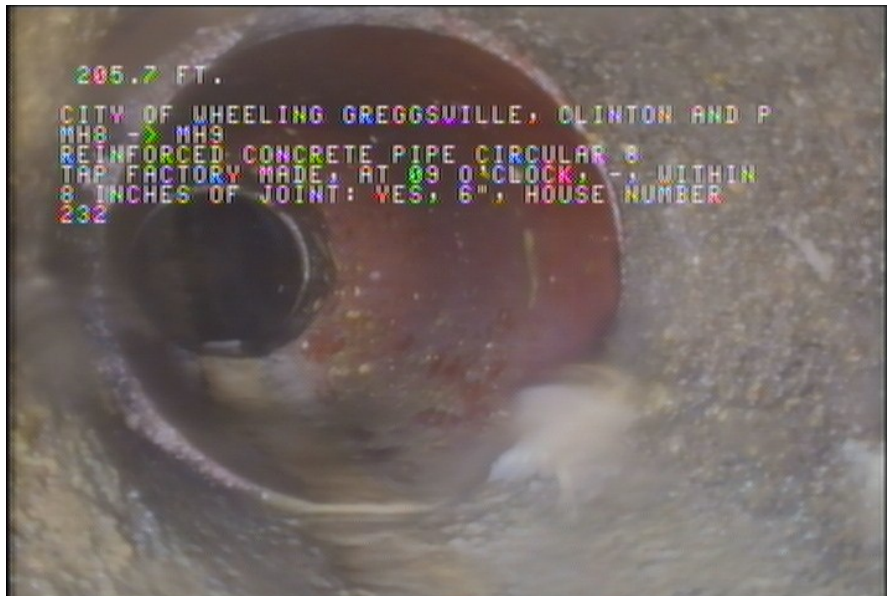
4, 00:09:50, 205.70ft Tap Factory Made, at 09 o'clock, -, within 8 inches of joint: YES, 6" / HOUSE NUMBER 232
