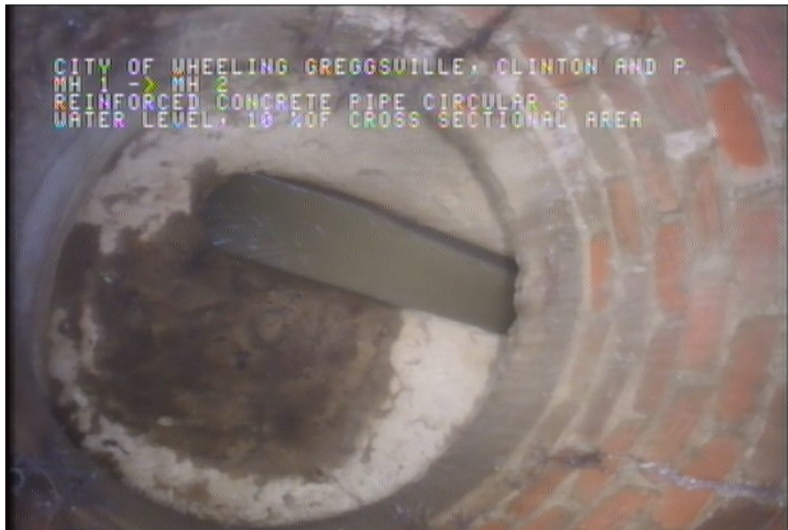
2, 00:00:00, 0.00ft Water Level, 10 % of cross sectional area
