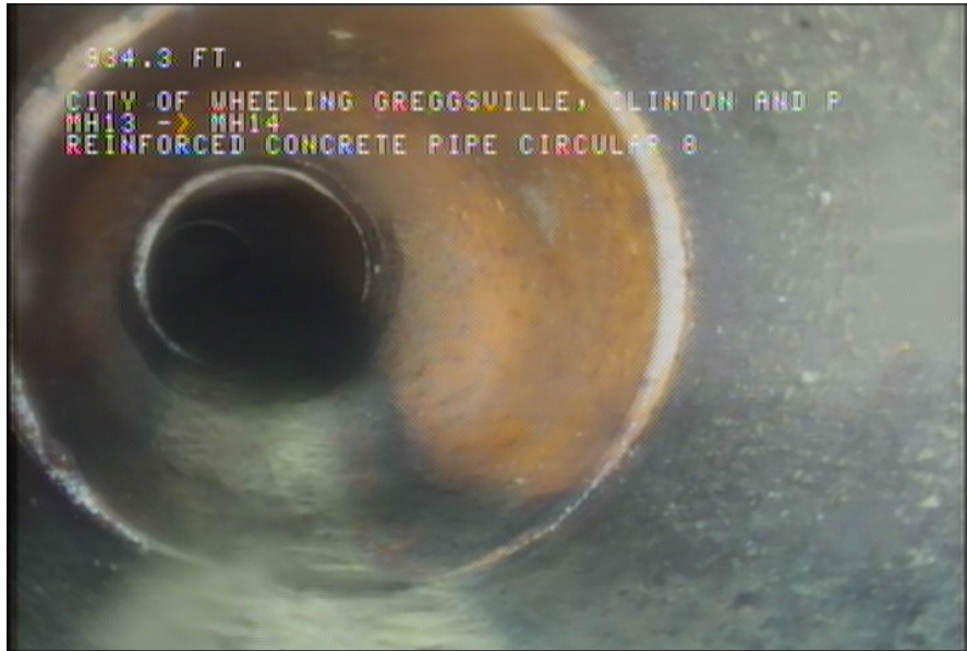
17, 00:32:28, 934.30ft Tap Factory Made, at 09 o'clock, -, within 8 inches of joint: YES, 6" / HOUSE NUMBER 160
