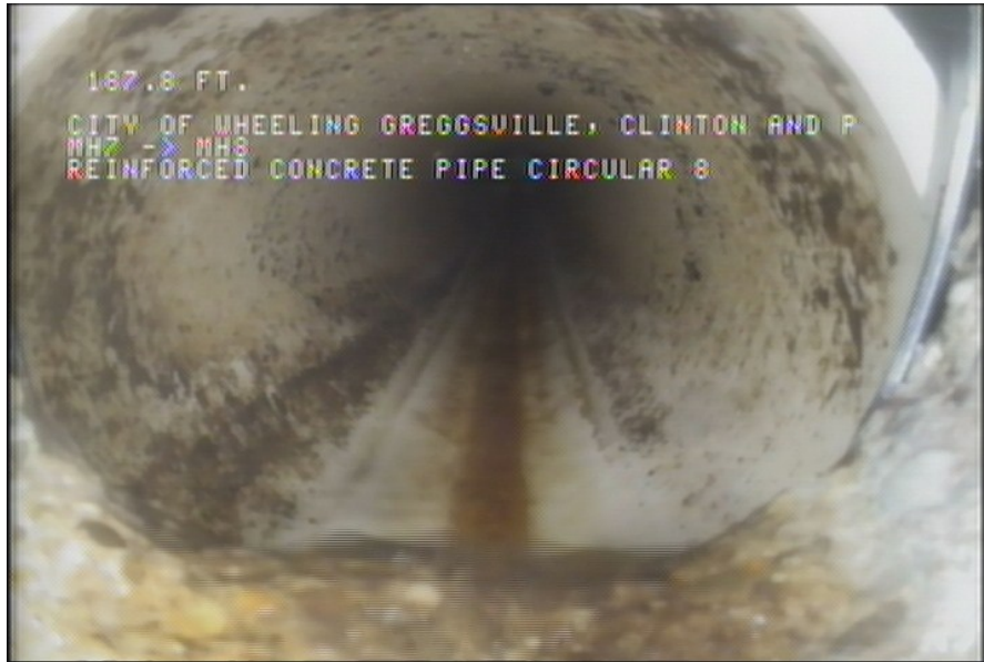
5, 00:09:02, 187.80ft Tap Break-In, at 09 o'clock, -, within 8 inches of joint: YES, 4" / HOUSE NUMBER 240A
