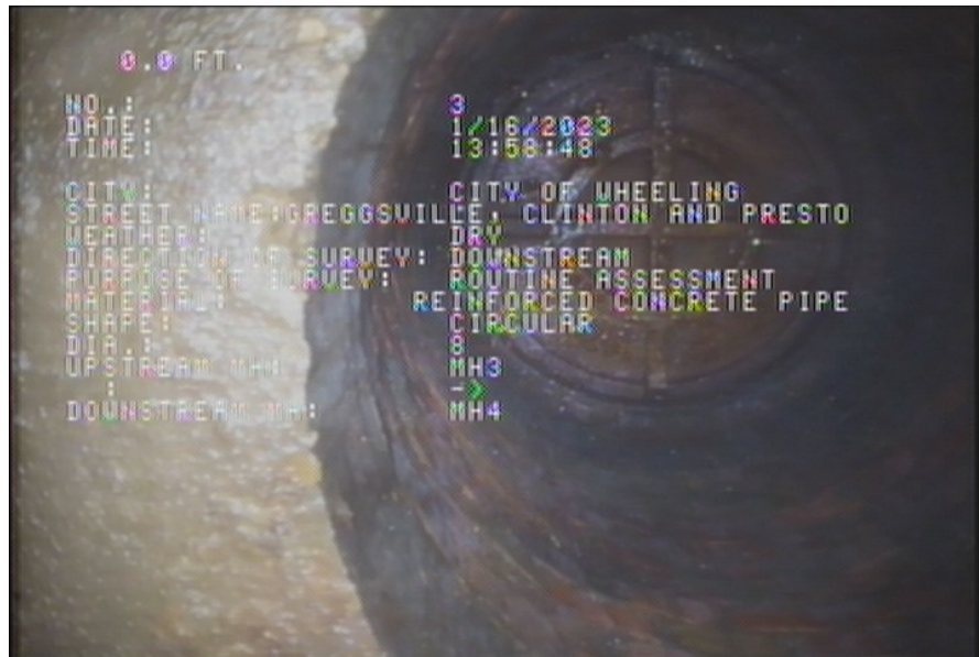
1, 00:00:00, 0.00ft Upstream Manhole, Survey Begins / MH3
