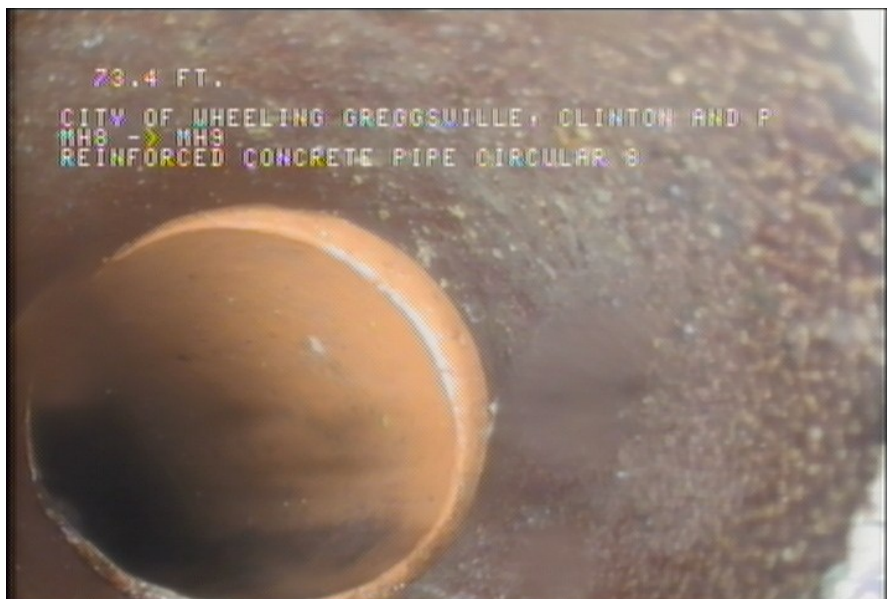
2, 00:03:40, 73.00ft Tap Break-In, at 10 o'clock, -, within 8 inches of joint: YES, 4" / HOUSE NUMBER 236
