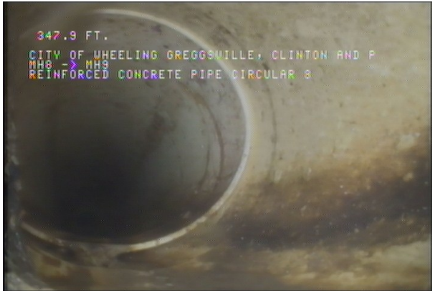
7, 00:18:03, 347.90ft Tap Break-In, at 10 o'clock, -, within 8 inches of joint: YES, 4" / HOUSE NUMBER 228
