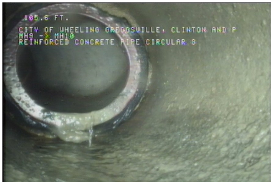
2, 00:04:49, 105.60ft Tap Factory Made, at 09 o'clock, -, within 8 inches of joint: YES, 6" / HOUSE NUMBER 222
