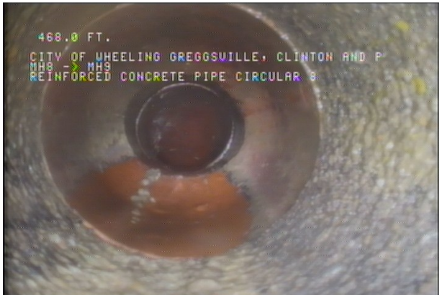
8, 00:24:18, 468.00ft Tap Factory Made, at 11 o'clock, -, within 8 inches of joint: YES, 6" / HOUSE NUMBER 224
