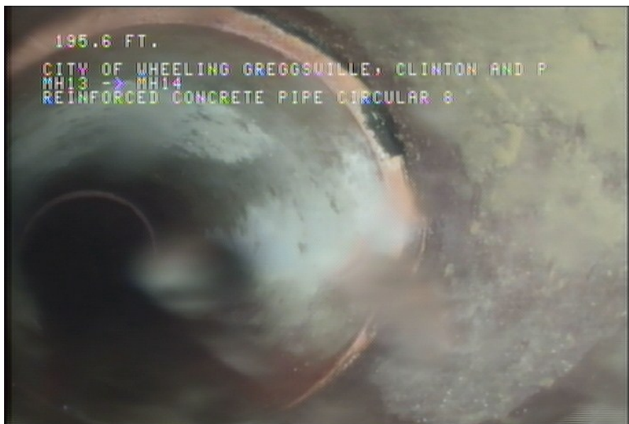
4, 00:11:44, 195.60ft Tap Factory Made, at 09 o'clock, -, within 8 inches of joint: YES, 6" / HOUSE NUMBER 182
