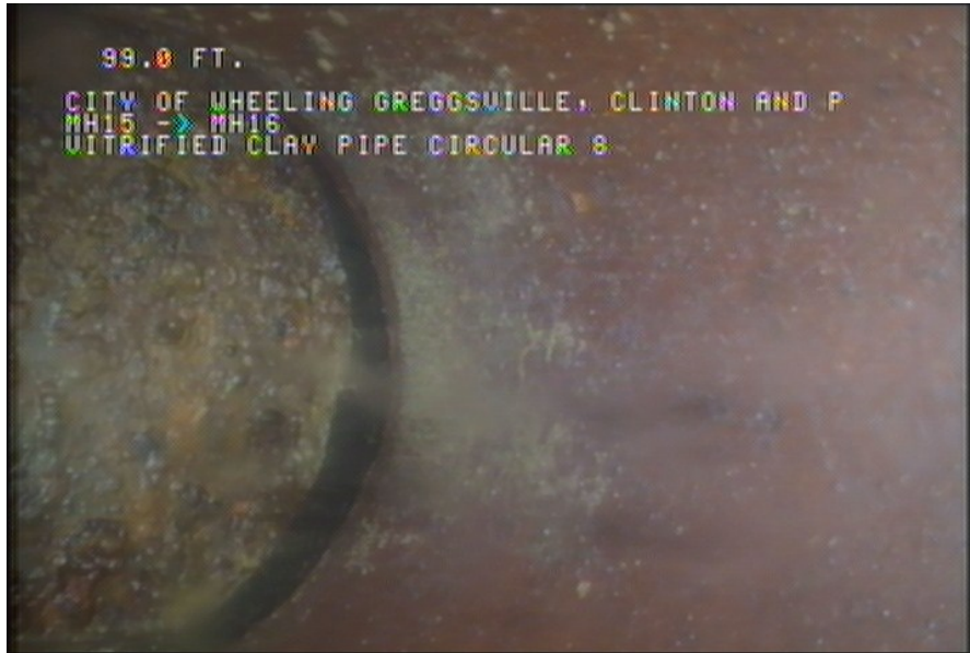
3, 00:06:58, 99.00ft Tap Factory Made Capped, at 09 o'clock, -, within 8 inches of joint: YES, 6"
