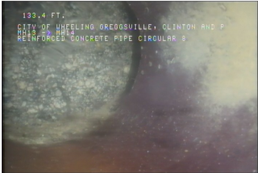
3, 00:08:49, 133.40ft Tap Factory Made Capped, at 09 o'clock, -, within 8 inches of joint: YES, 6"
