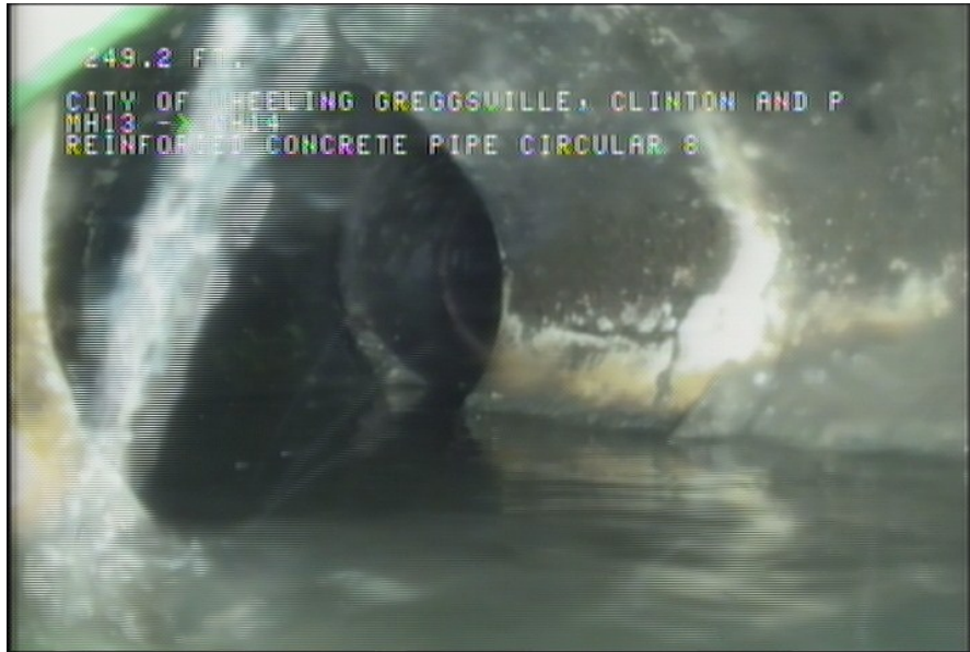
5, 00:18:45, 249.30ft Tap Break-In, at 09 o'clock, -, within 8 inches of joint: YES, 6" / HOUSE NUMBER 180
