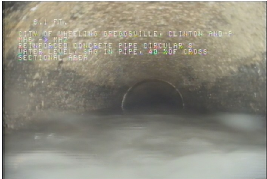
3, 00:05:37, 6.10ft Water Level, Sag in pipe, 40 % of cross sectional area / HEAVY CLEAN
