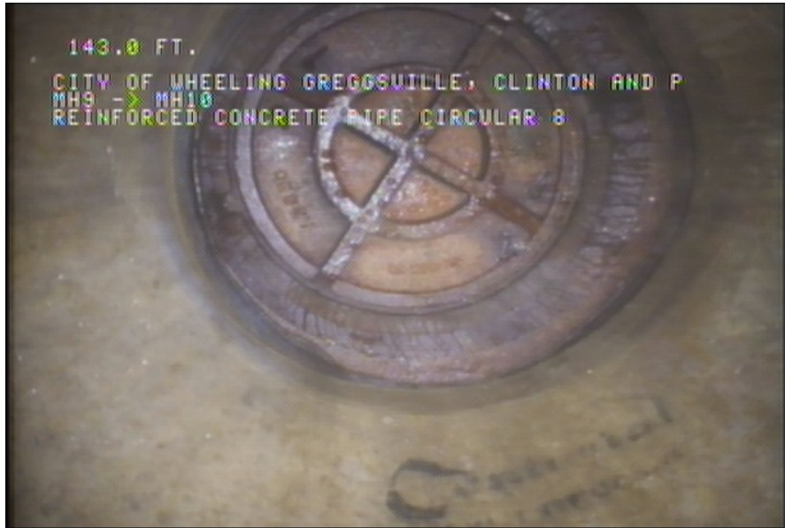
3, 00:07:14, 143.00ft Downstream Manhole, Survey Ends / MH10
