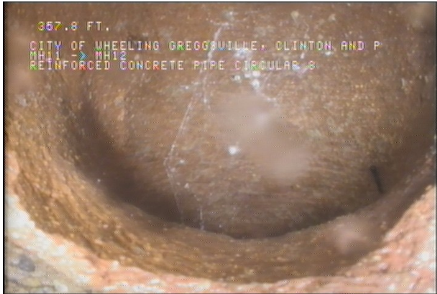
9, 00:26:57, 357.80ft Tap Break-In, at 12 o'clock, -, within 8 inches of joint: YES, 4" / HOUSE NUMBER 200
