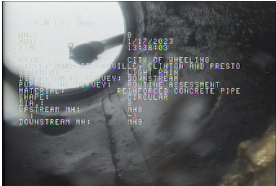
1, 00:00:00, 0.00ft Upstream Manhole, Survey Begins / MH8
