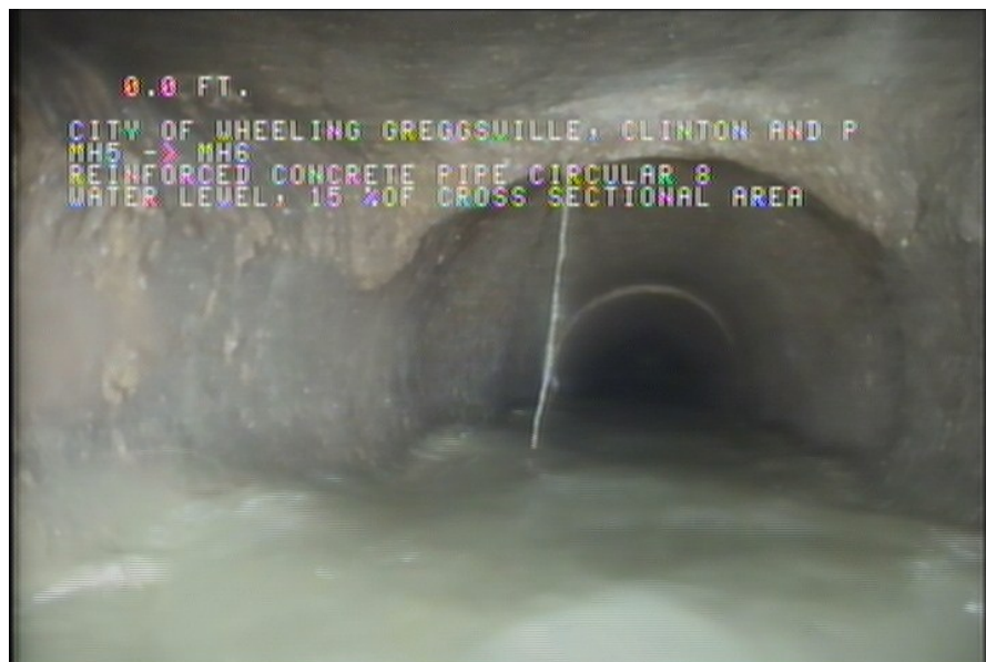
2, 00:00:35, 0.00ft Water Level, 15 % of cross sectional area
