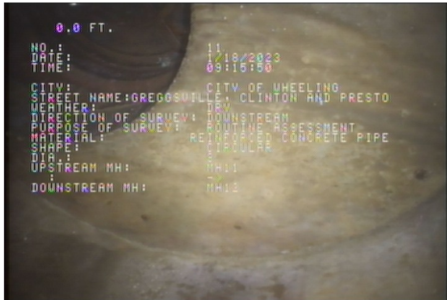
1, 00:00:00, 0.00ft Upstream Manhole, Survey Begins / MH11
