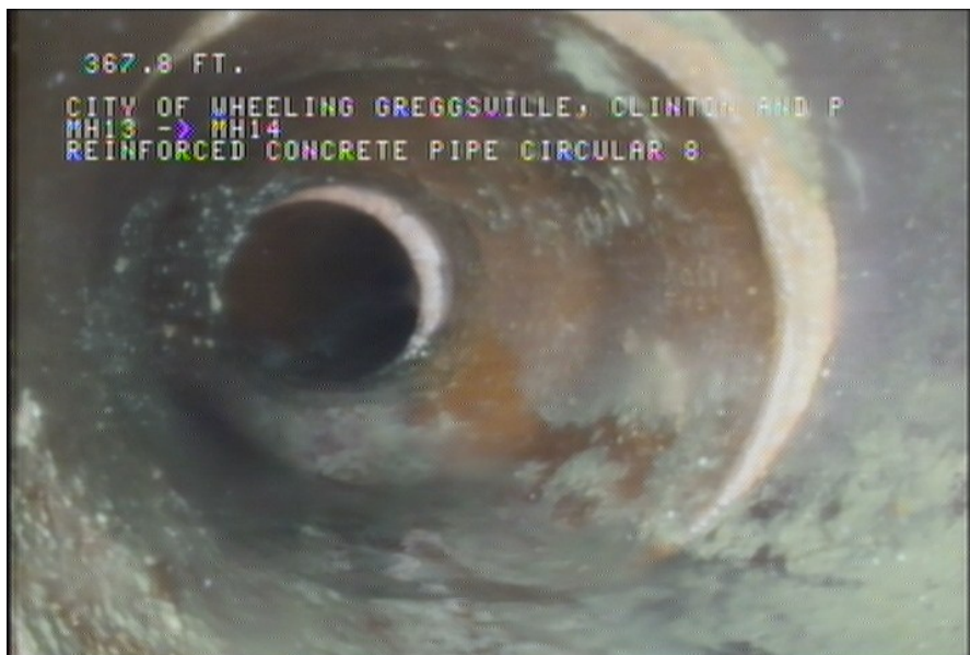
8, 00:28:09, 367.80ft Tap Factory Made, at 09 o'clock, -, within 8 inches of joint: YES, 6" / HOUSE NUMBER 176
