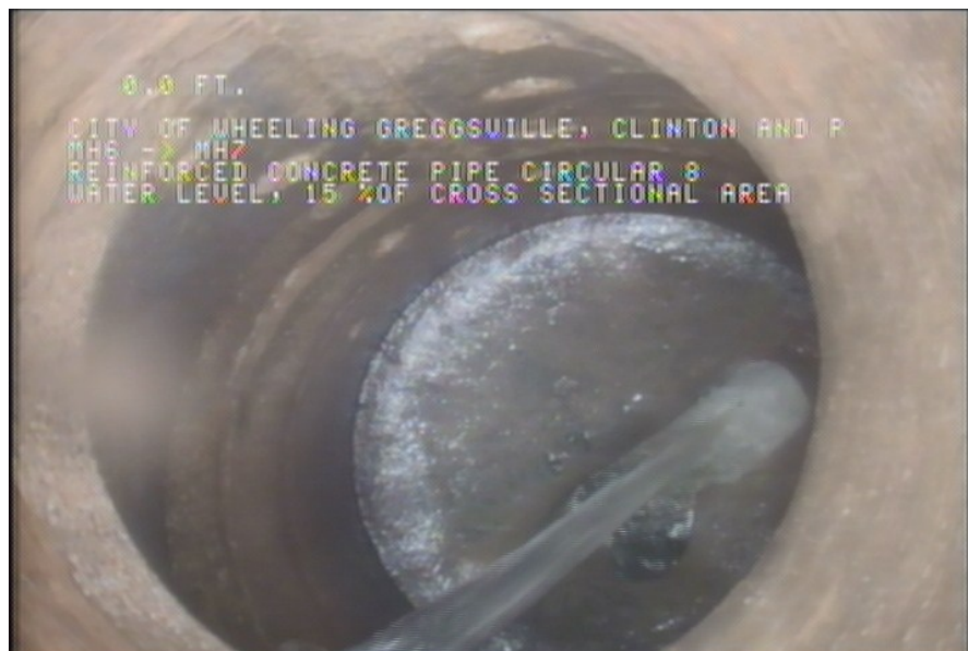
2, 00:00:27, 0.00ft Water Level, 15 %of cross sectional area
