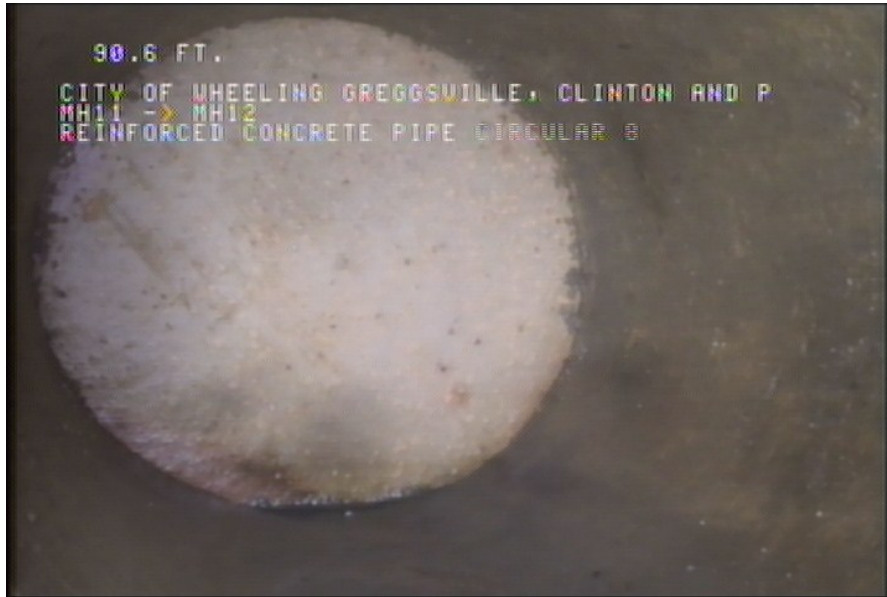
3, 00:06:23, 90.60ft Tap Factory Made Capped, at 09 o'clock, -, within 8 inches of joint: YES, 6"
