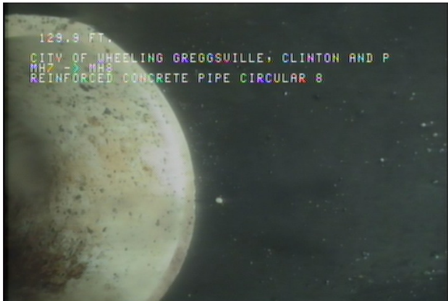
4, 00:05:55, 129.90ft Tap Break-In, at 10 o'clock, -, within 8 inches of joint: YES, 4" / HOUSE NUMBER 240B
