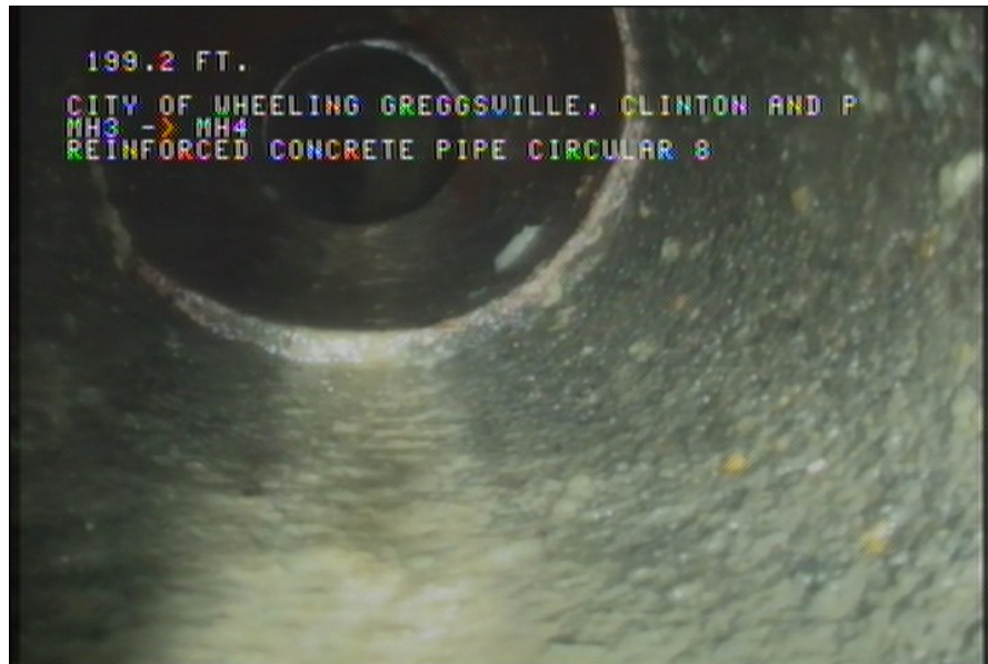
5, 00:18:45, 199.20ft Tap Factory Made, at 09 o'clock, -, within 8 inches of joint: YES, 6" / HOUSE NUMBER 268
