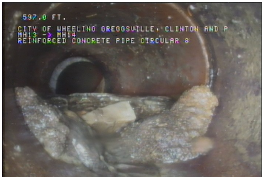
12, 00:44:12, 597.00ft Tap Factory Made, at 09 o'clock, -, within 8 inches of joint: YES, 6" / HOUSE NUMBER 168
