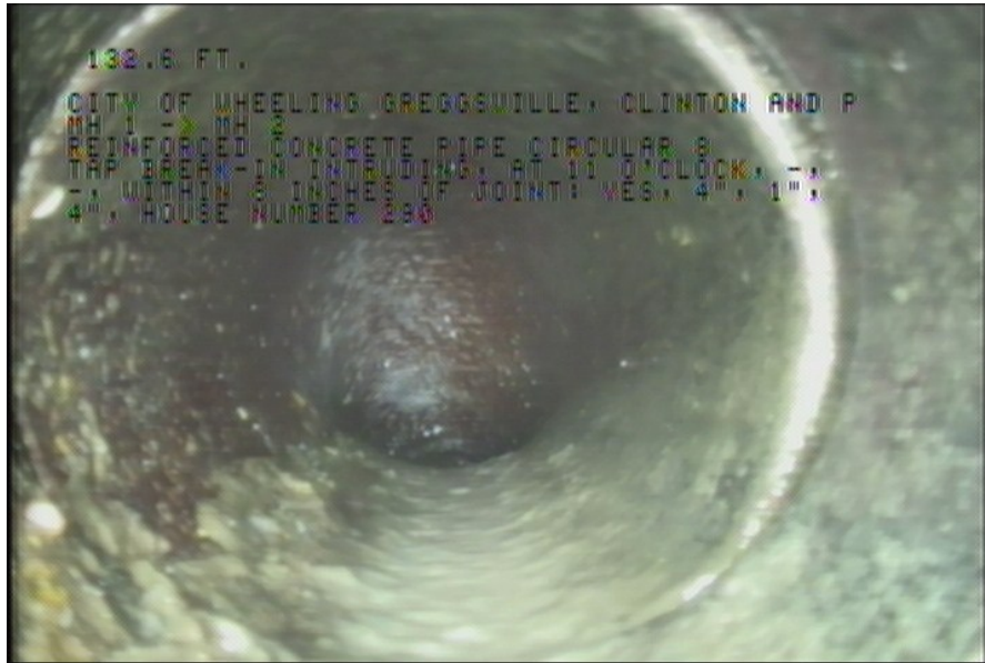
3, 00:00:00, 132.60ft Tap Break-In Intruding, at 11 o'clock, -, -, within 8 inches of joint: YES, 4", 1", 4" / HOUSE NUMBER 290
