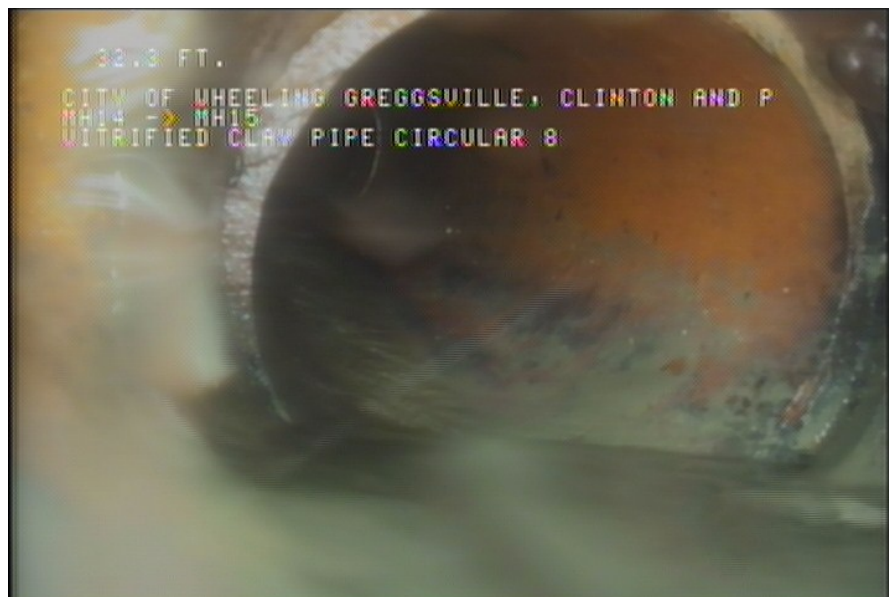
2, 00:06:00, 32.30ft Tap Factory Made, at 09 o'clock, -, within 8 inches of joint: YES, 6" / HOUSE NUMBER 158
