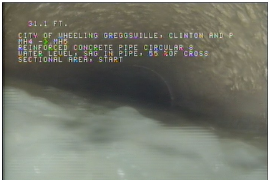
2, 00:02:36, 31.10ft Water Level, Sag in pipe, 55 %of cross sectional area, Start
