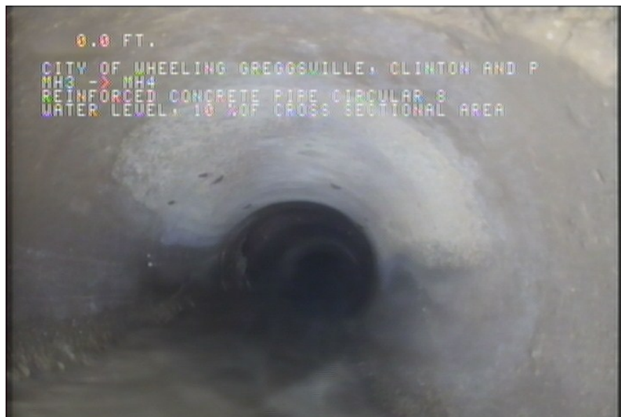
2, 00:00:30, 0.00ft Water Level, 10 % of cross sectional area
