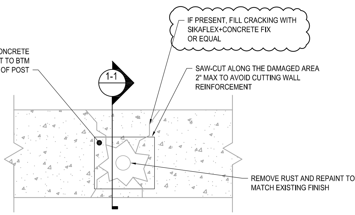
NEW WORK PLAN VIEW
