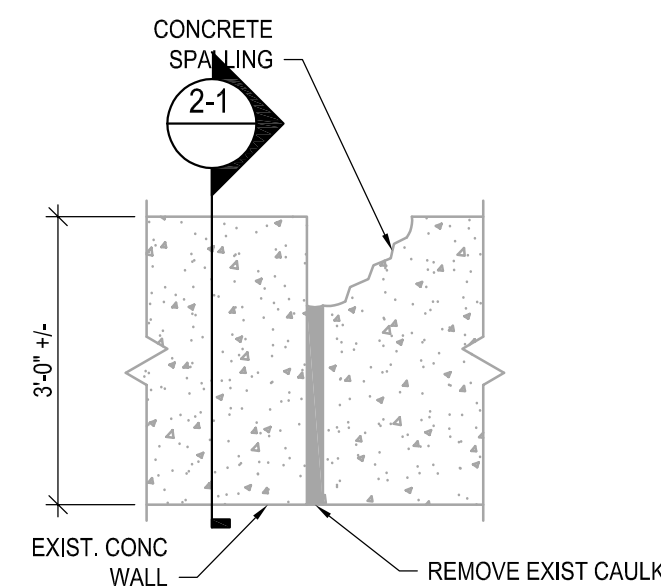
EXIST ELEVATION VIEW
