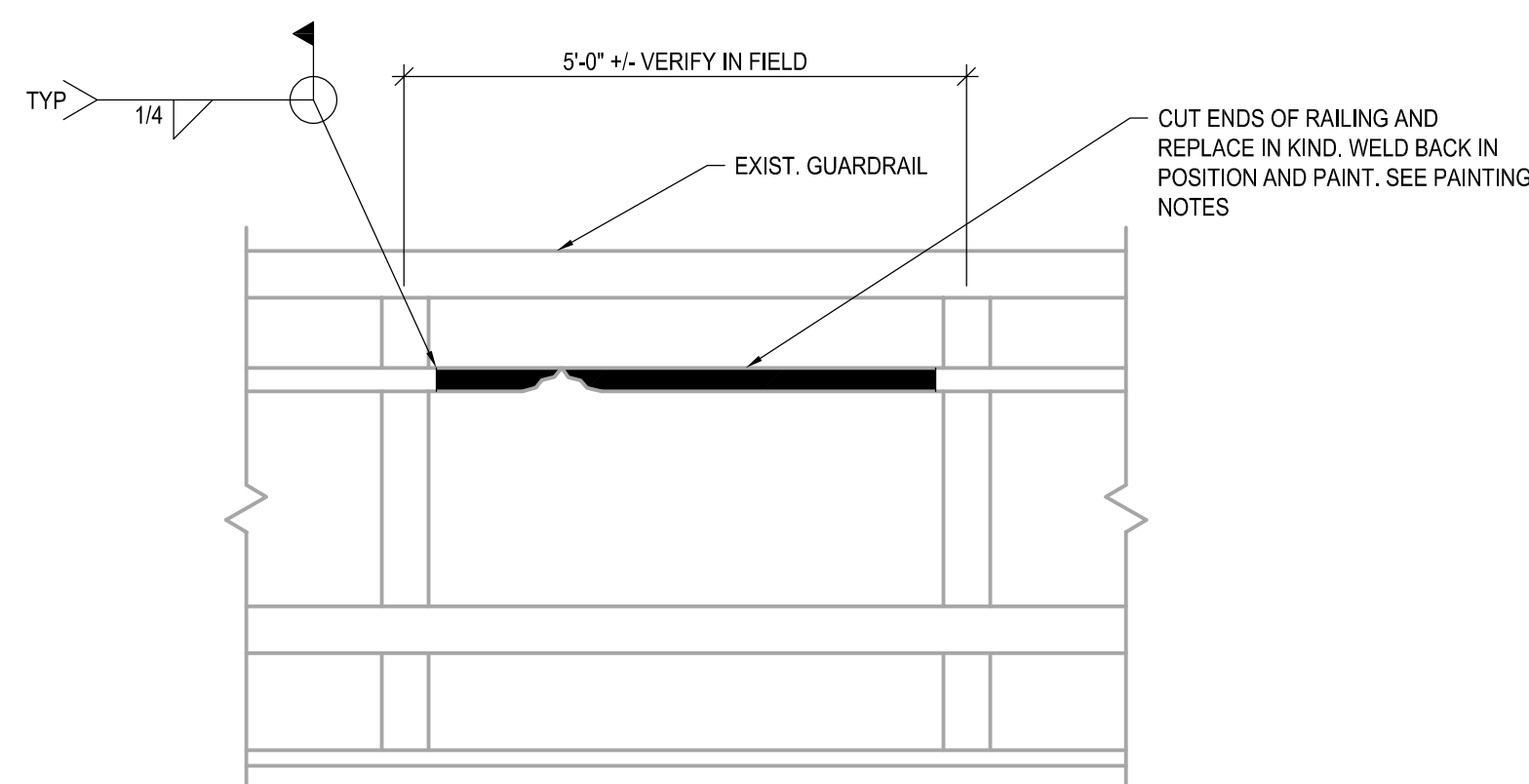
4 GUARDRAIL REPAIR - DETAIL 4 S103 SCALE: 1/2" = 1'-0"
