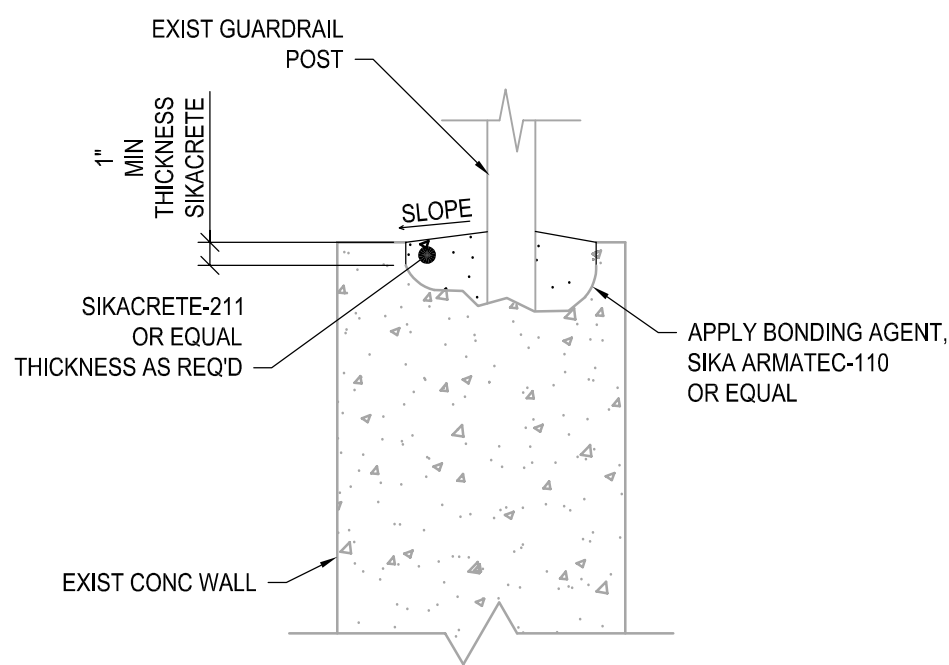
1-1 SECTION S103 SCALE: 3/4" = 1'-0"
