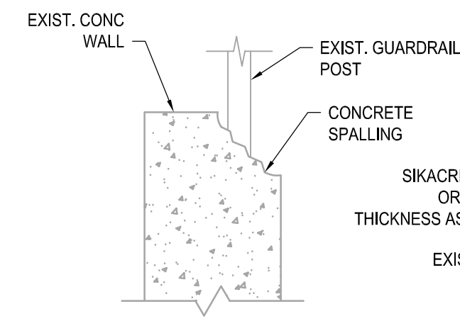
3-1 EXIST SECTION S103
