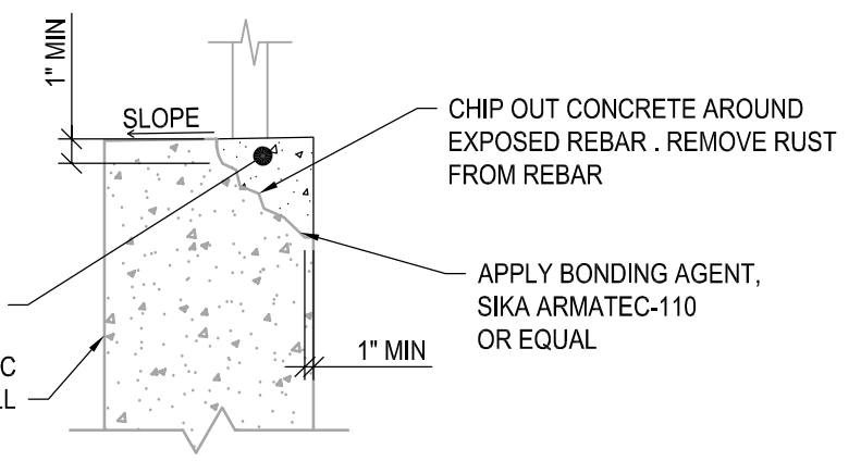
3-2 NEW WORK SECTION S103
