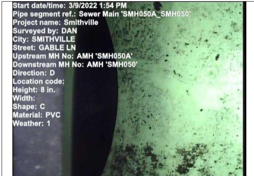
At: 0 ft. AMH - Manhole Joint: No SMH050A
