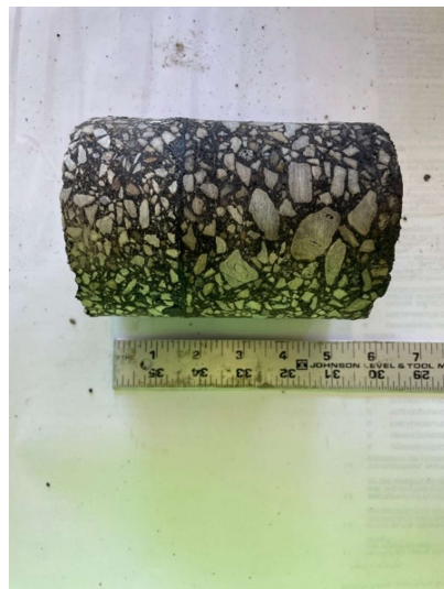
CORE SAMPLE
