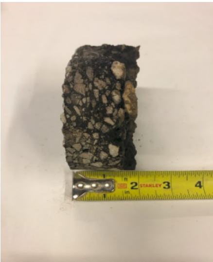
CORE SAMPLE
